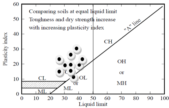
Figure 5 Plasticity chart for laboratory classification of fine grained soils
